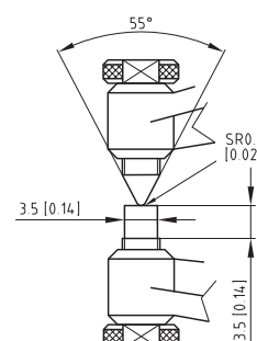
Contact Point Type 4
