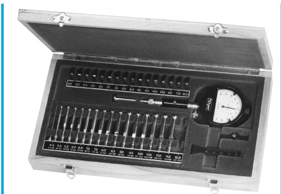
200-140 Complete set with indicator. Indicator not included with set. Order indicator separately.
