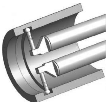
Ball Contacts Ø 5 mm
