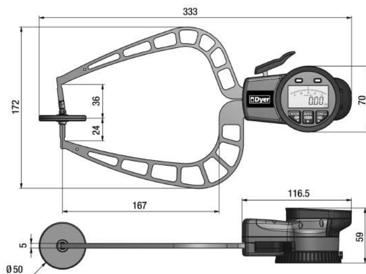
Electronic Model 306-851
