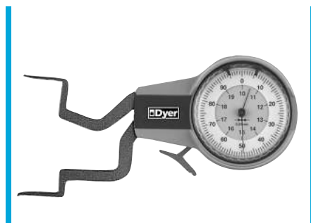
104 Series Special Arms and Contacts Measure ID and OD groove at bottom of a hub within a bore.
