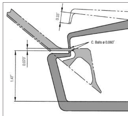
Hard-to-reach Min-Wall
