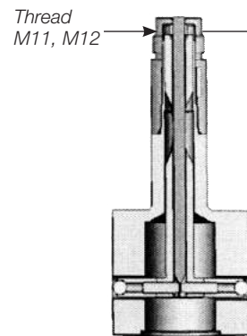
Thru bore small sleeve design
