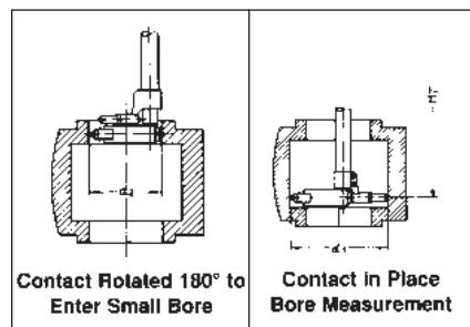
Contact rotates 180°
