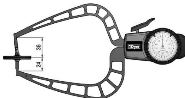
Mechanical Model 306-821
