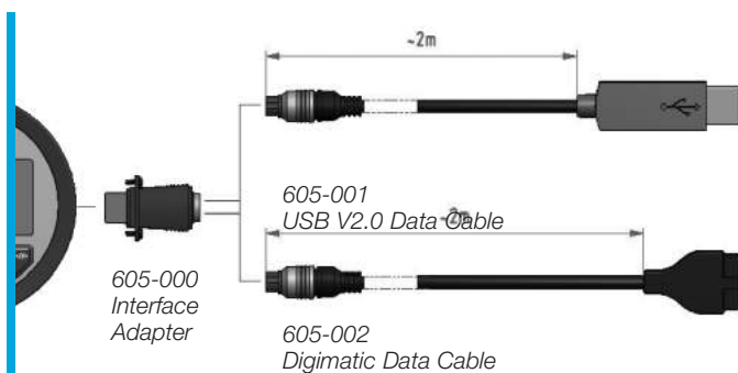
SPC Cables
