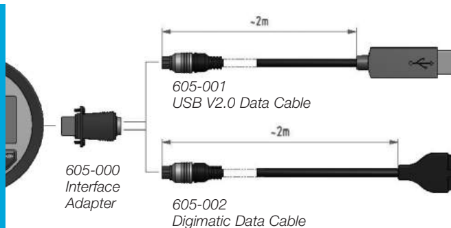
SPC Cables
