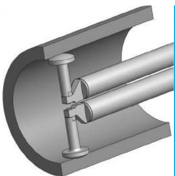
Mushroom Type R Ø 20 mm
