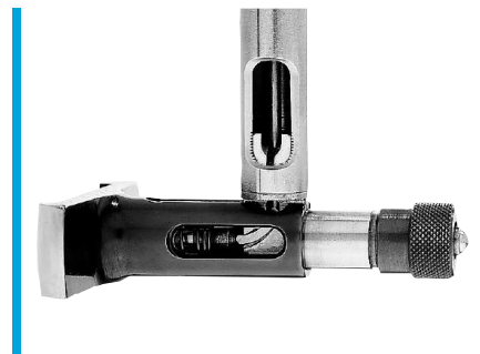
Transfer system in measuring head
