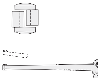
101-105 Modified Special range 0.240"-0.800" (6-20 mm), special scissor contacts with 0.200" radius x 150° wide (5 x 4 mm) and special reach 3.25" (82 mm)
