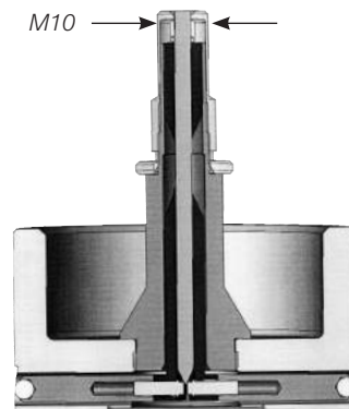
Large sleeve design
