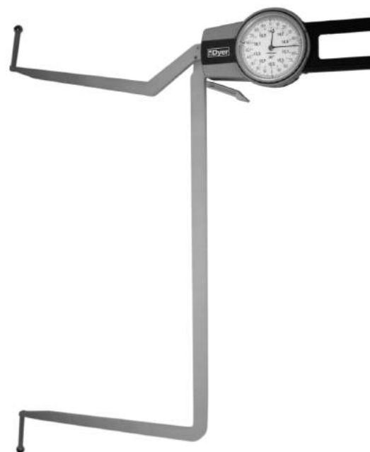
Modified 101 Series with special larger measuring range.
