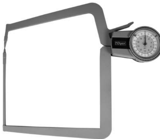
302 Special Extra long lower contact to clear part range.
